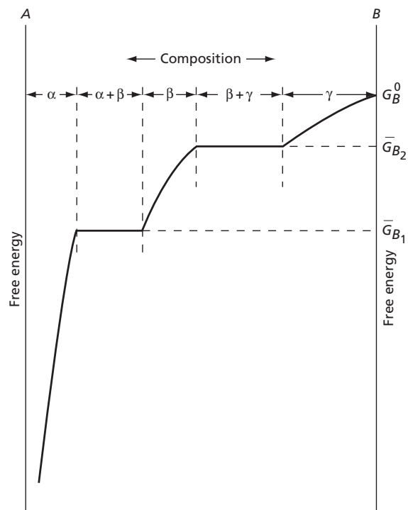
FIG. 12.27 The variation of \bar{G}_B with composition across the phase diagram at T_1
