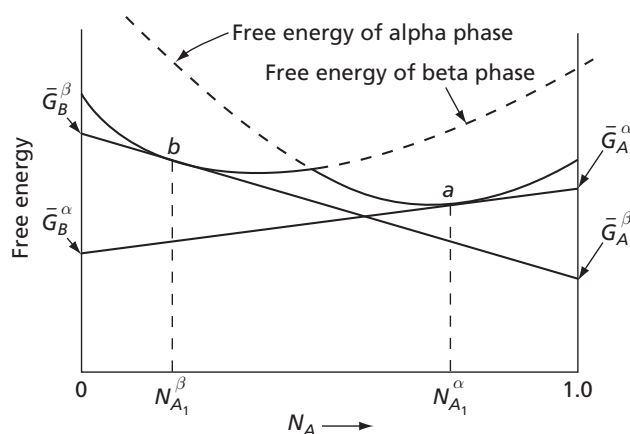
FIG. 10.9 Two phases having compositions of N_{A1}^\alpha and N_{A1}^\beta , respectively, cannot be in equilibrium
