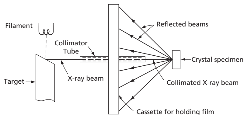
FIG. 2.5 Laue back-reflection camera
