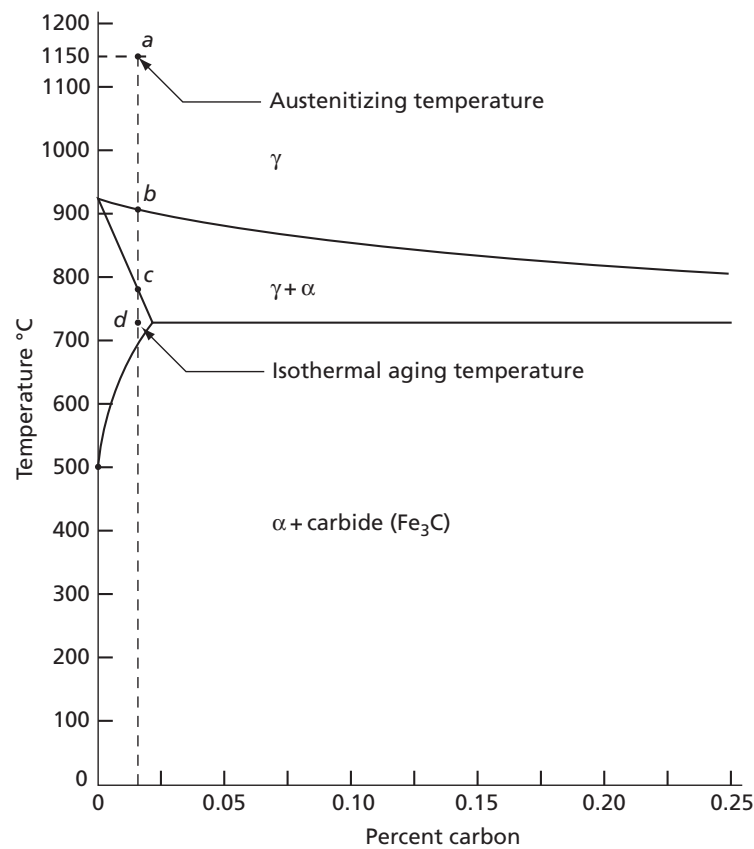
FIG. 16.15 A partial view of the iron-carbon diagram
