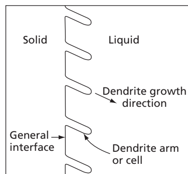
FIG. 14.20 Schematic representation of the first stage of dendritic growth. A temperature inversion is assumed to exist at the interface; that is, the temperature in the liquid drops in advance of the interface
