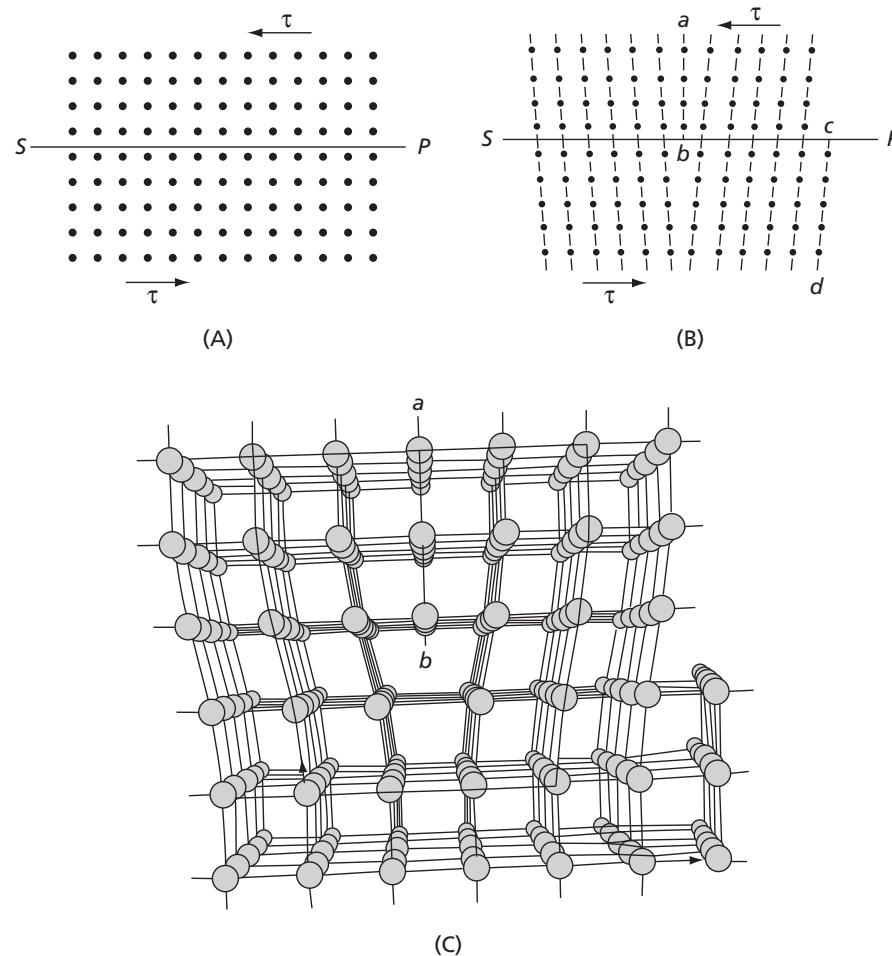
FIG. 4.7 An edge dislocation. (A) A perfect crystal. (B) When the crystal is sheared one atomic distance over part of the distance S-P , an edge dislocation is formed. (C) Three dimensional view of slip
