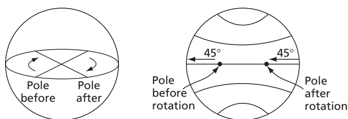
FIG. 1.29 The rotation of the pole of the (1\bar{1}0) plane is given here. The diagram on the left shows the rotation in a perspective figure, whereas that on the right shows the motion of the pole along a latitude line of a stereographic projection which, in this case, is the equator
