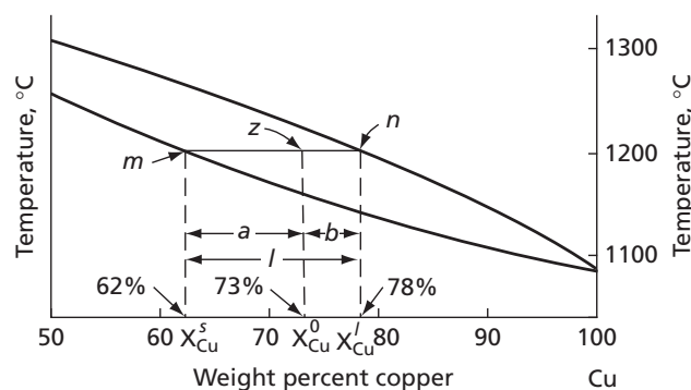
FIG. 11.2 The lever rule
