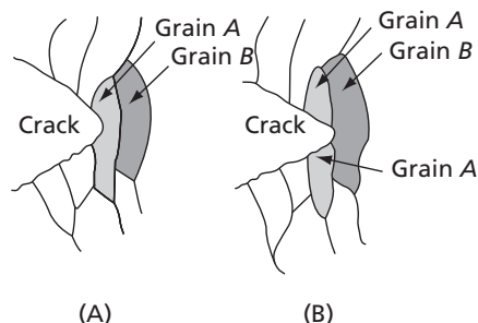
FIG. 21.26 Propagation of a ductile fracture according to Rogers.
