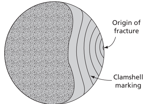
FIG. 21.31 Fatigue fractures in machinery parts subjected to stress cycles that vary in magnitude with time are liable to show a clamshell pattern in the burnished area
