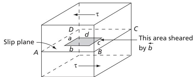
FIG. 4.17 A closed dislocation loop consisting of (a) positive edge, (b) right-hand screw, (c) negative edge, and (d) left-hand screw
