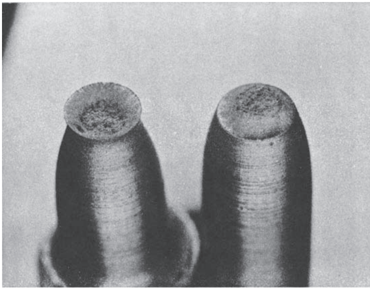
FIG. 21.18 Cup and cone fracture
