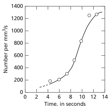
FIG. 18.18 Rate of nucleation ( N ) of pearlite as a function of time. Eutectoid steel transformed at 680°C. (Mehl, R. F., and Dube, A., Phase Transformations in Solids , John Wiley and Sons, Inc., New York, 1951, p. 545.)
