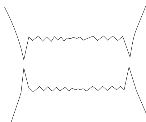
FIG. 21.27 Double cup fracture.
