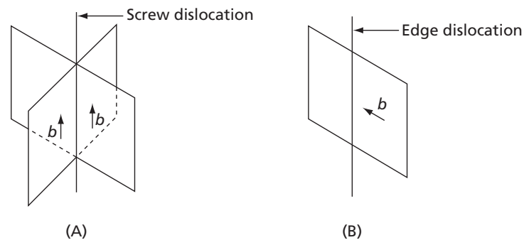
FIG. 4.28 (A) Any plane containing the dislocation is a slip plane for a screw dislocation. (B) There is only one slip plane for an edge dislocation. It contains both the Burgers vector and the dislocation
