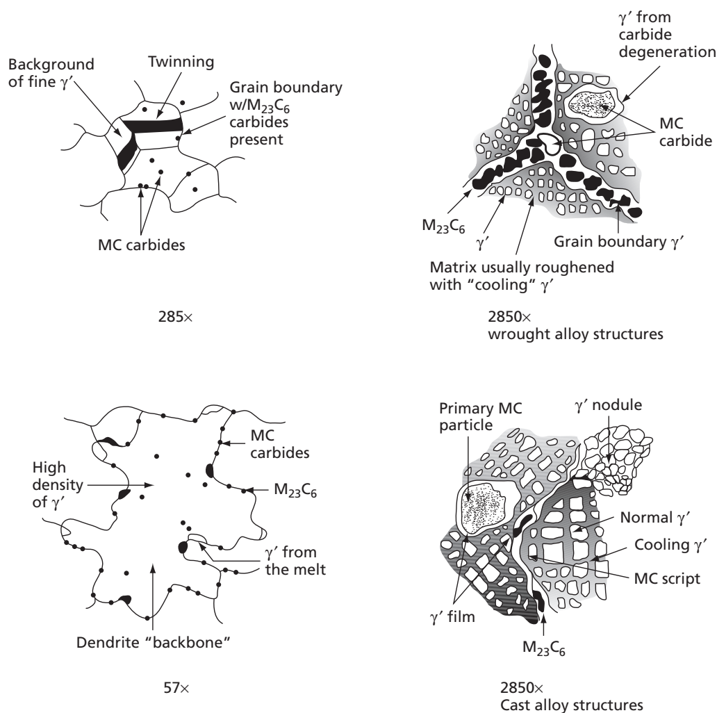
FIG. 20.21 Structures characteristic of wrought (top) and cast (bottom) nickel-base superalloys. (From Sims, C. T., and Hagel, W. C., The Superalloys , John Wiley and Sons, Inc., New York, 1972. Reprinted with permission of John Wiley & Sons, Inc.)
