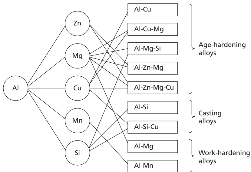
FIG. 20.7 Major aluminum alloy systems (Hatch, J.E., Ed., Aluminum: Properties and Physical Metallurgy , © 1984. Reprinted with permission of ASM International (R). All rights reserved. www.asminternational.org )
