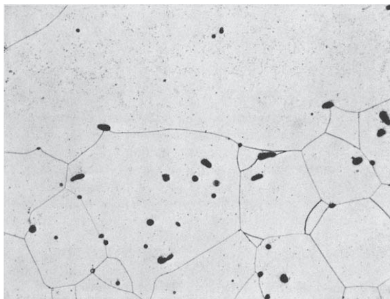
FIG. 8.37 Interaction between pores and grain boundaries
