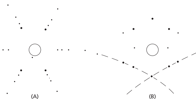
FIG. 2.6 Laue back-reflection photographs. (A) Photograph with X-ray beam perpendicular to the basal plane (0001). (B) Photograph with X-ray beam perpendicular to a prism plane (11 \bar{2} 0). Dashed lines on the photograph are drawn to show that the back-reflection spots lie on hyperbolas
