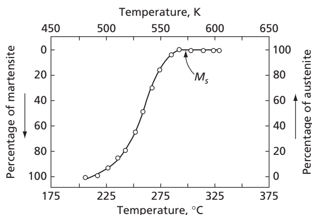
FIG. 19.15 The formation of martensite in a 0.40 percent carbon low-alloy steel (2340) as a function of temperature. (After Grange, R. A., and Stewart, H. M., Trans. AIME , 167 467 [1946].)
