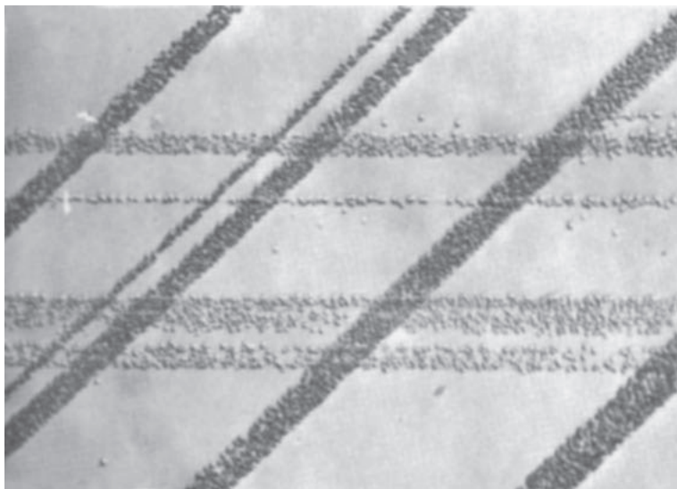
FIG. 5.24 Slip bands in LiF. Bands formed at -196\text{ }^{\circ}\text{C} and 0.36 percent strain (Reprinted with permission from J.J. Gilman and W.G. Johnson, Journal of Applied Physics , Vol. 30, Issue 2, Page 129, Copyright 1959, American Institute of Physics)
