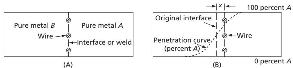
FIG. 12.6 Marker movement in a Kirkendall diffusion couple
