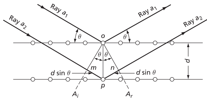
FIG. 2.2 The Bragg law
