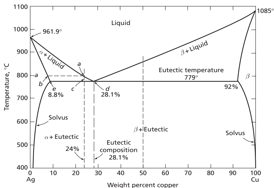
FIG. 11.13 Copper-silver phase diagram. (From Constitution of Binary Alloys , by Hansen, M., and Anderko, K. Copyright, 1958. McGraw-Hill Book Co., Inc., New York, p. 18. Used by permission.)
