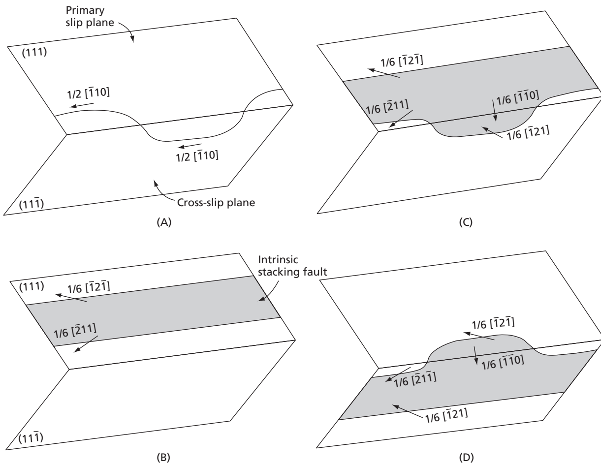
FIG. 5.26 The cross-slip of an extended dislocation
