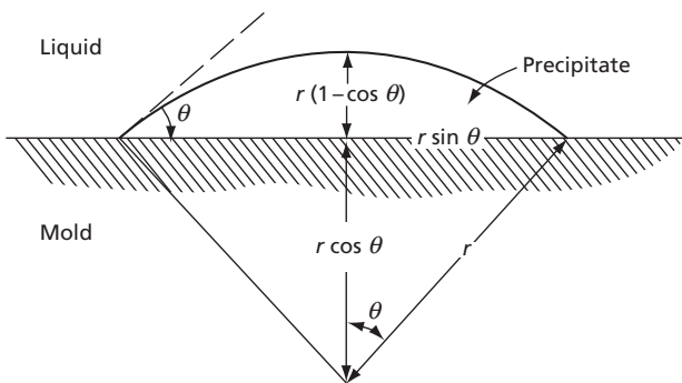
FIG. 15.12 A hypothetical spherical cap embryo
