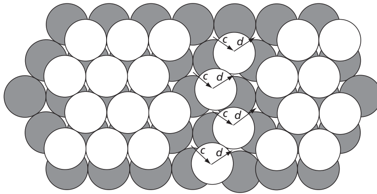
FIG. 4.23 Partial dislocation in a face-centered cubic lattice
