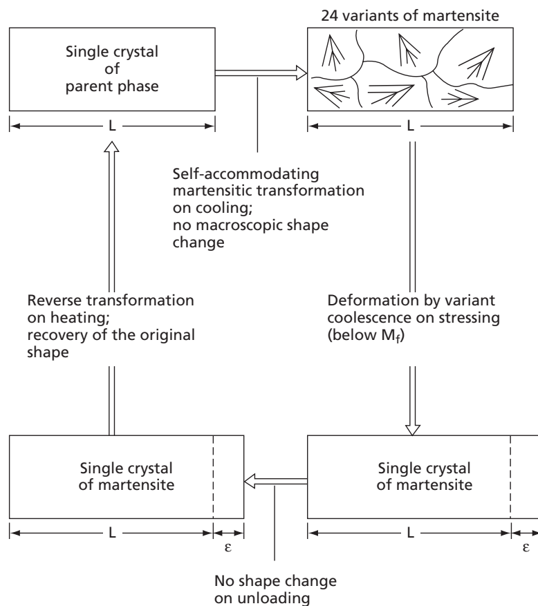
FIG. 17.42 A schematic diagram illustrating the shape-memory processes. (From Wayman, C. M., Solid → Solid Phase Transformations , Aaronson, H. I., Loughin, D. E., Sekerka, R. F., and Wayman, C. M., Eds., p. 1138, Met. Soc. AIME , Warrendale, Pa., 1981 p. 1138, Figure 12.)
