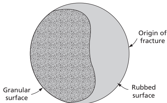
FIG. 21.30 The surface of a fatigue fracture usually shows two regions with characteristically different aspects. One is smooth, or burnished, corresponding to the slow spreading of the fatigue crack, and the other is rough, or granular, belonging to the metal that failed as a result of overload
