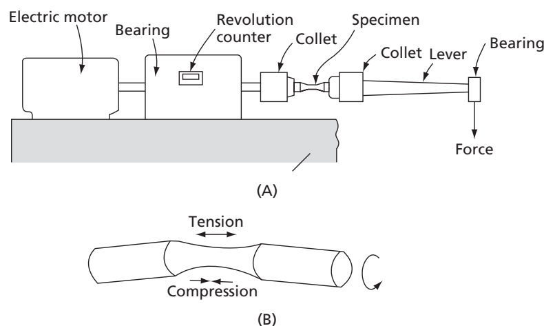
FIG. 21.32 (A) One form of rotating-beam fatigue-testing machine. (B) Fatigue-test specimen. Specimen is bent while it rotates. Any point in the reduced middle section alternates between states of tensile and compressive stress
