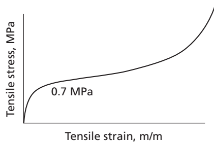
FIG. 4.1 Tensile stress-strain curve for a magnesium single crystal
