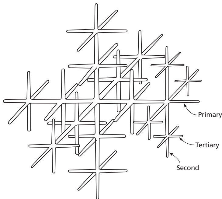
FIG. 14.33 A dendritic crystal formed by three-dimensional dendritic growth. Tertiary arms are shown on one set of secondary arms only (see right side of figure). (After Grignon {1775} and Tschernoff {1878}.)
