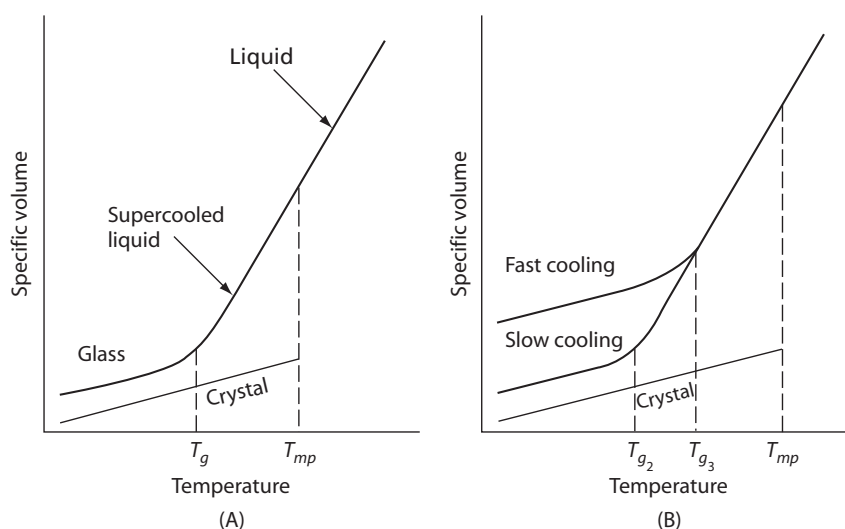
FIG. 14.6 Specific volume of liquid, glass, and crystal versus temperature
