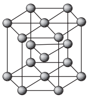
FIG. 1.6 The close-packed hexagonal unit cell
