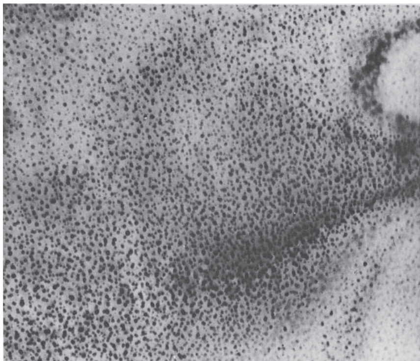
FIG. 16.8 Guinier-Preston zones in an aluminum 16 percent silver alloy. (Reprinted from Nicholson, R.B., and Nutting, J., Acta. Met. 9 332 [1961] with permission of Elsevier. Photograph courtesy of RB Nicholson. http://www.sciencedirect.com/science/journal/00016160 )
