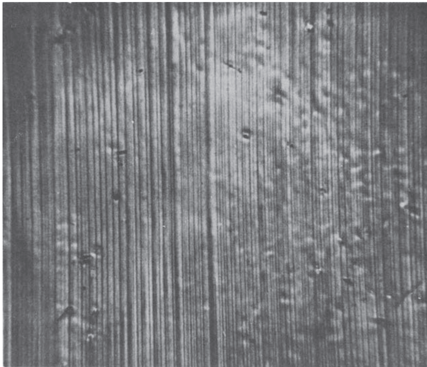
FIG. 17.33 Twinned structure (tetragonal) in an indium-thallium alloy after transformation. (Burkart, M. W., and Read, T. A., Trans. AIME , 197 1516 [1953].)
