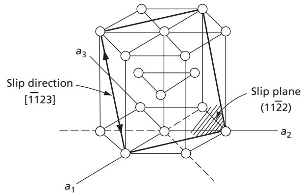
FIG. 5.18 \{11\bar{2}2\} \langle 11\bar{2}3 \rangle slip in hexagonal metals
