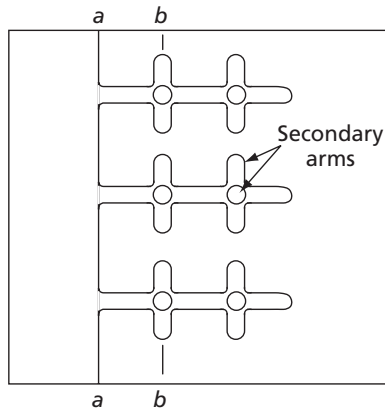
FIG. 14.22 In a cubic crystal, the dendrite arms form along \langle 100 \rangle directions. Primary and secondary arms are thus normal to each other
