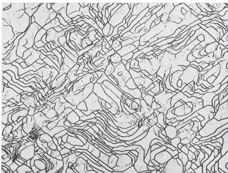
FIG. 8.15 Complex polygonized structure in a silicon-iron single crystal that was formed 8 percent by cold rolling before it was annealed 1 hr at 1373 K. (From Hibbard, W.R. Jr, and Dunn, ASM Seminar, Creep and Recovery , 1957, p. 52 Reprinted with permission of ASM International(R). All rights reserved. www.asminternational.org )
