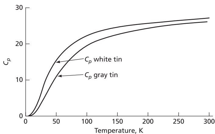
FIG. 10.1 C_p as a function of temperature for both forms of solid tin
