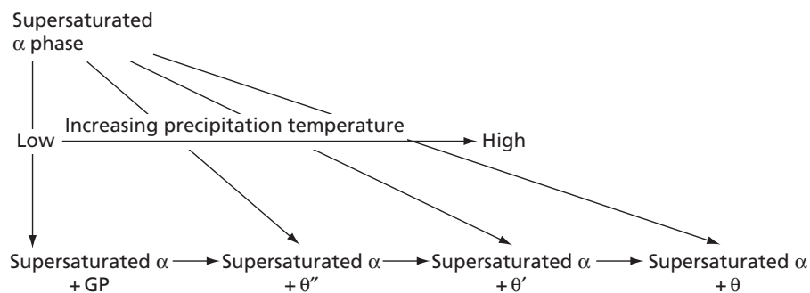
FIG. 16.12 Precipitation sequence in Al-Cu alloys
