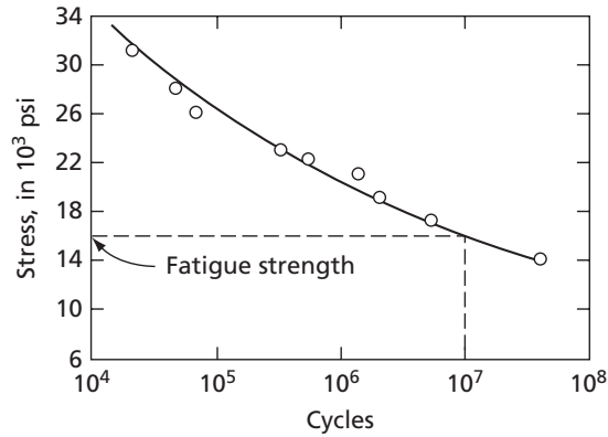
FIG. 21.34 A typical S - N curve for a nonferrous metal (aluminum alloy). (From Prevention of Fatigue of Metals , p. 48, The Staff of the Battelle Memorial Institute, John Wiley and Sons, Inc., New York, 1941.)
