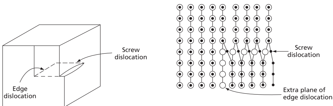
FIG. 4.15 Atomic configuration corresponding to the dislocation of Fig. 4.14 viewed from above. Open-circle atoms are above the slip plane, dot atoms are below the slip plane
