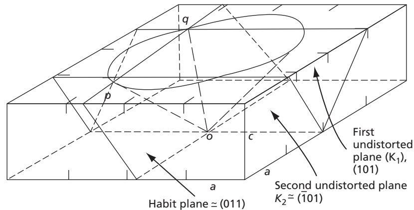
FIG. 17.28 Positions of the two undistorted planes, K_1 and K_2 , in the indium-thallium martensite transformation
