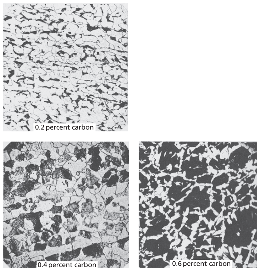
FIG. 18.34 Hypoeutectoid-steel microstructures. Black areas are pearlite, white areas are ferrite. Approximately 300×
