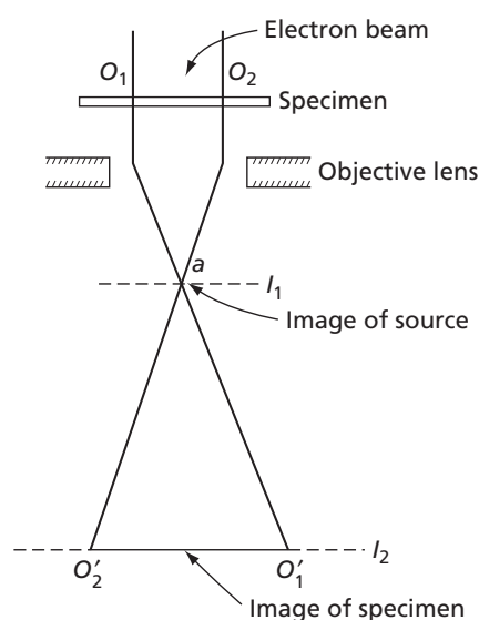
FIG. 2.16 Schematic drawing of a transmission electron microscope
