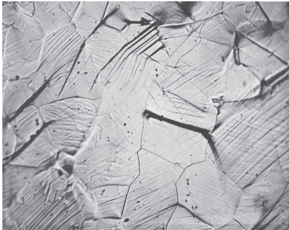
FIG. 21.13 A cleavage crack that stops at the boundaries of a single grain in a polycrystalline iron specimen. 200 \times (Hahn, G. T., Averbach, B. L., Owen, W. S., and Cohen, M., Fracture , p. 91, The Technology Press and John Wiley and Sons, Inc., New York, 1959.)
