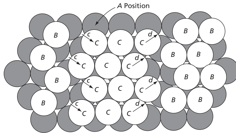
FIG. 4.25 An extended dislocation
