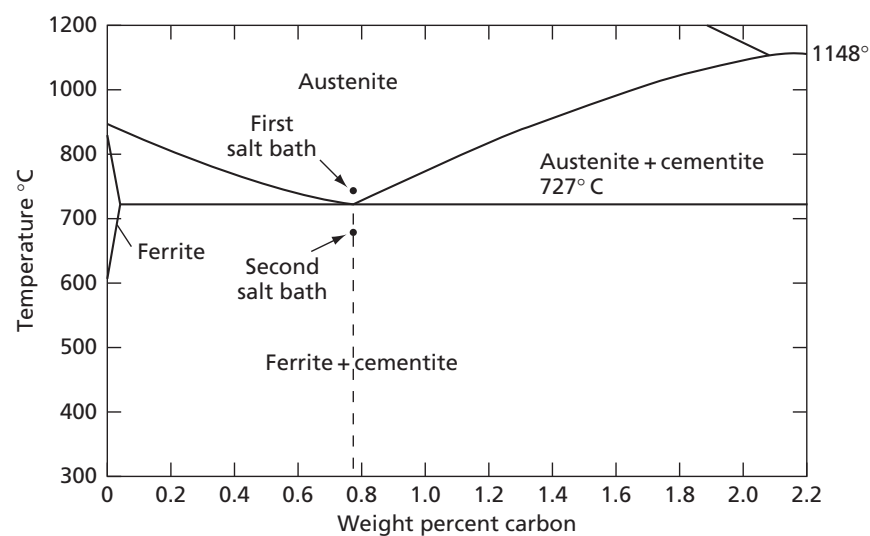
FIG. 18.5 The eutectoid section of the iron-carbon diagram
