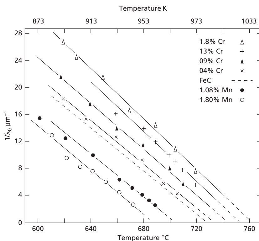
FIG. 18.16 Minimum interlamellar spacing data for eutectoid steel containing additions of manganese and chromium. (From Ridley, N., Met. Trans. A , 15A 1019 [1984] with kind permission from Springer Science and Business Media.)
