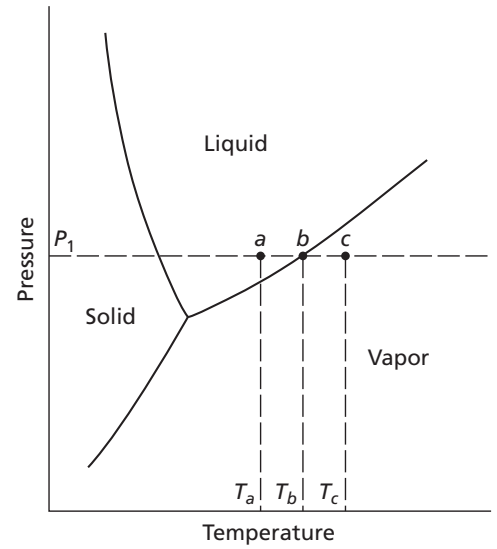
FIG. 15.4 A one-component (temperature-pressure) phase diagram
