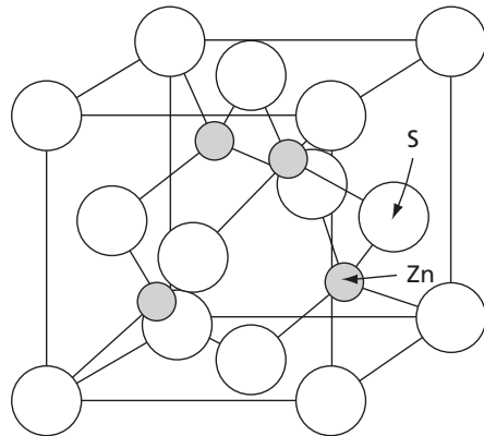
FIG. 3.3 The zincblende lattice, ZnS
