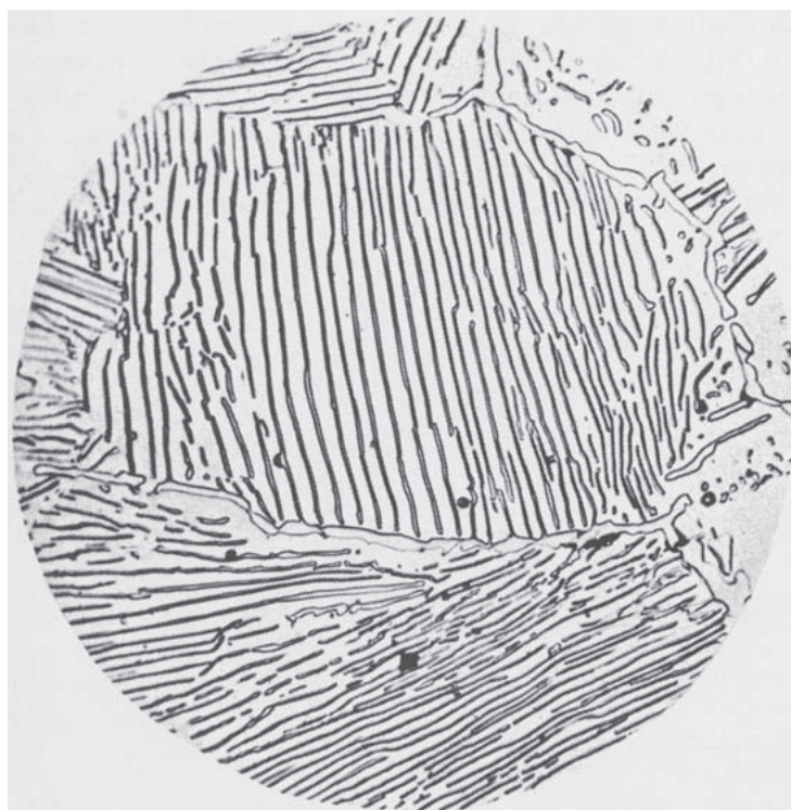
FIG. 18.36 Hypereutectoid-steel microstructure. Notice the band of cementite plates outlining the pearlite colony in the center of the photograph. 1000 \times
