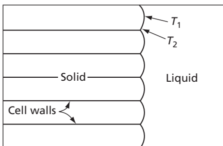
FIG. 14.29 When the region of constitutional supercooling is narrow, a cellular structure may form as the result of the movement of a stable interface of the type shown above
