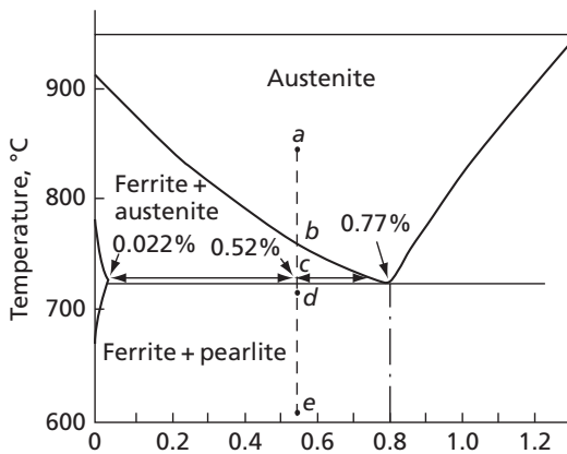
FIG. 18.32 Transformation of a hypoeutectoid steel on slow cooling
