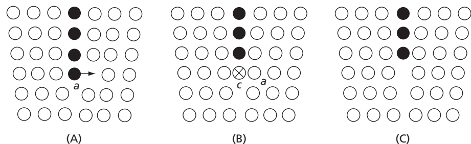
FIG. 4.29 Positive climb of an edge dislocation
