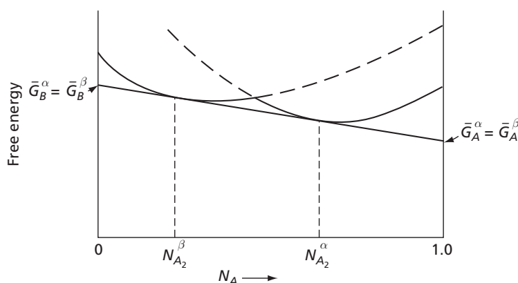
FIG. 10.10 Two phases in equilibrium
